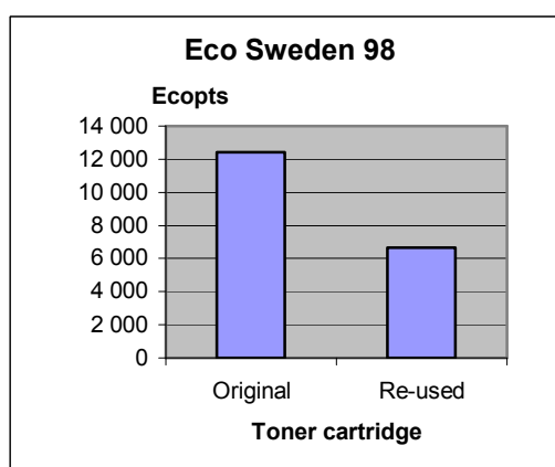
Figure 17. "Eco Sweden 98", alternative scenario, without paper
