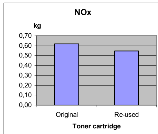
Figure 4. Emissions, NOx, main scenario, with paper
