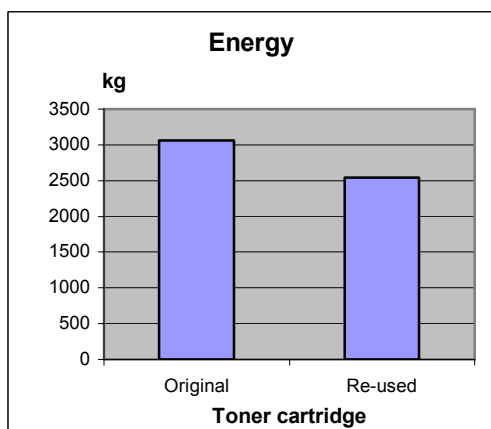
Figure 5. Total energy consumption main scenario, with paper
