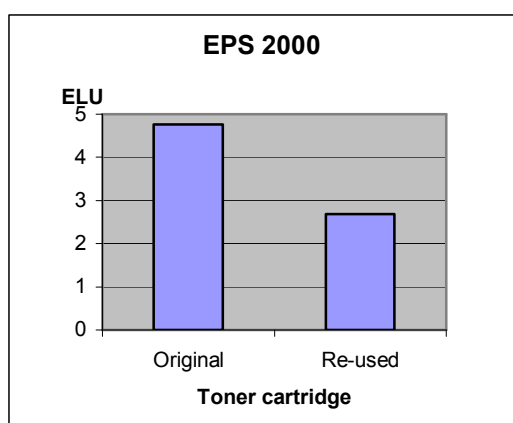
Figure 16. "EPS 2000", alternative scenario, without paper
