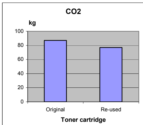
Figure 3. Emissions, CO2, main scenario, with paper
