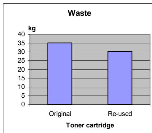
Figure 6. Total amount of waste main scenario, with paper
