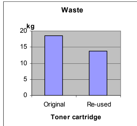
Figure 10. Total amount of waste, alternative scenario, without paper
