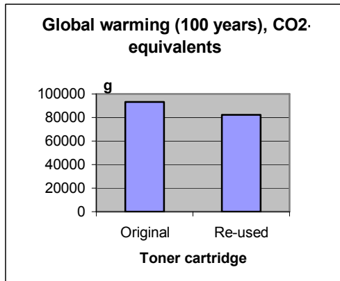
Figure 11. “Global warming (100 years)”, CO2-equivalents, scenario, with paper
