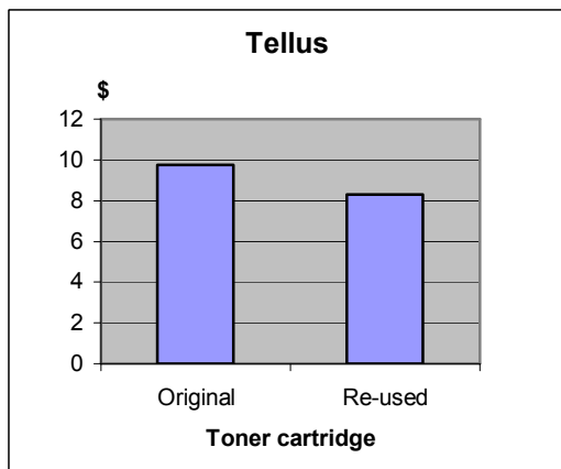
Figure 14. ”Tellus”, main scenario, with paper
