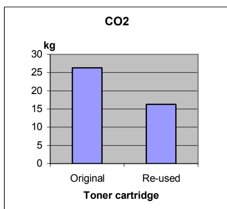
Figure 7. Emissions, CO 2 , alternative scenario, without paper
