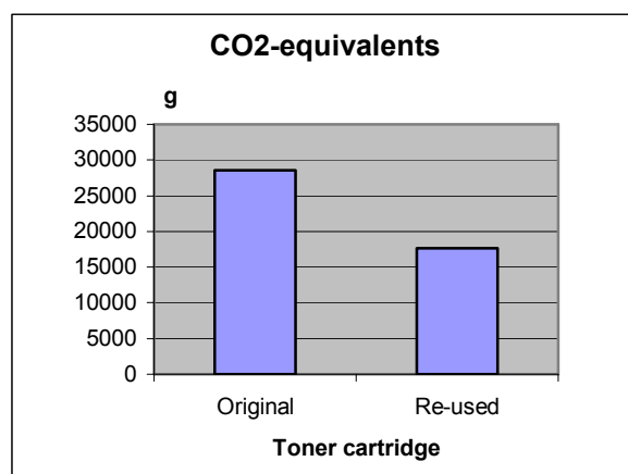
Figure 15. "Global warming (100 years)", CO2-equivalents, alternative scenario, without paper
