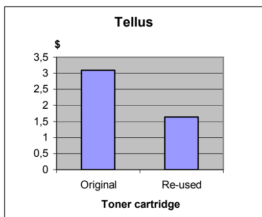
Figure 18. "Tellus", alternative scenario, without paper
