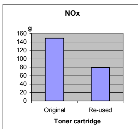
Figure 8. Emissions, NO x , alternative scenario, without paper
