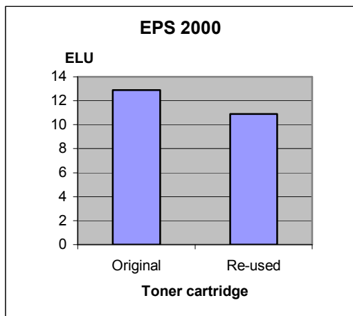
Figure 12. ”EPS 2000”, main scenario, with paper
