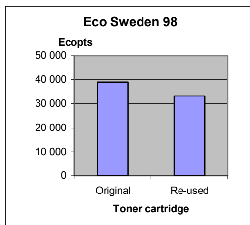
Figure 13. ”Eco Sweden 98”, main scenario, with paper
