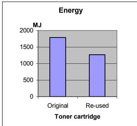
Figure 9. Total energy consumption alternative scenario, without paper
